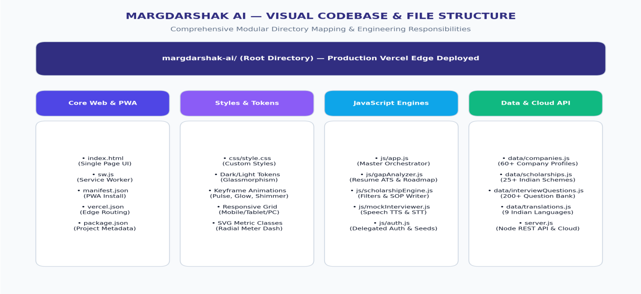
Figure 5: Visual Codebase Architecture & Modular File Responsibilities
