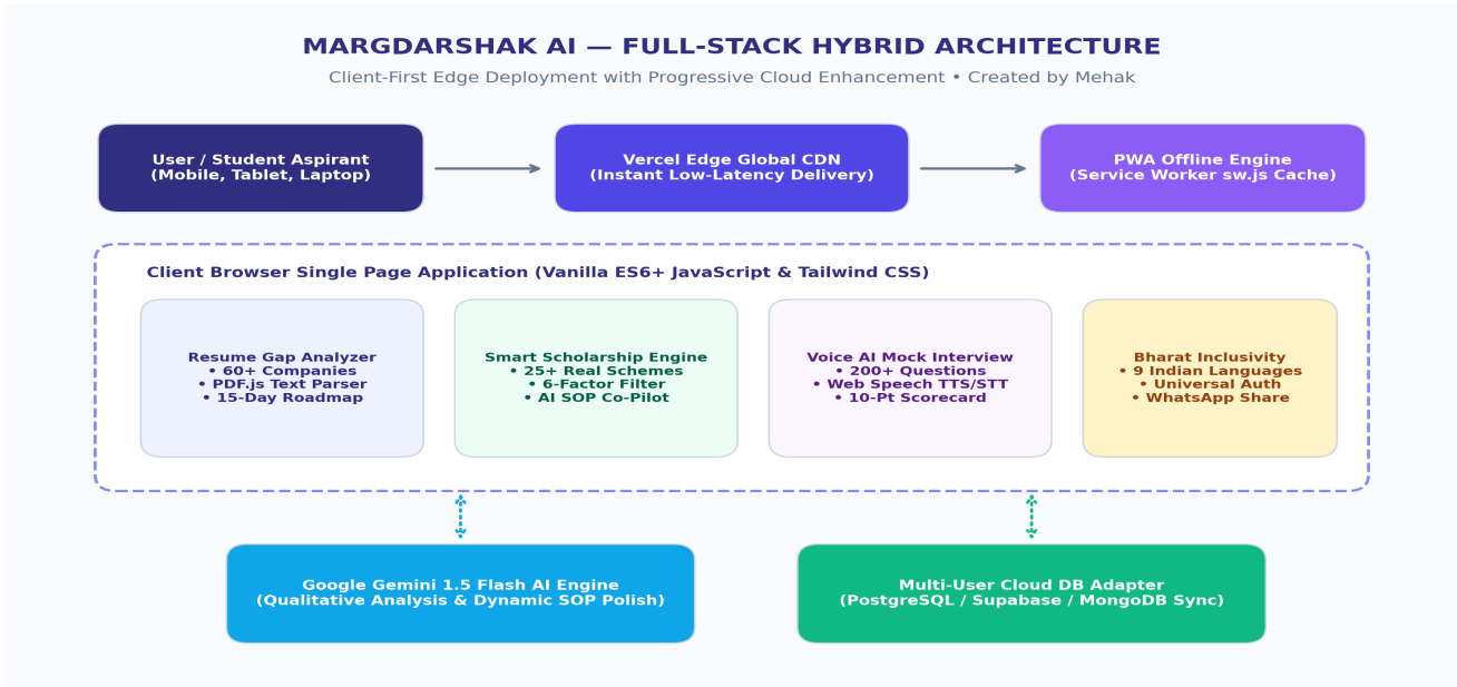
Figure 1: Full-Stack Hybrid Architecture — Client-First SPA + Progressive Cloud AI
