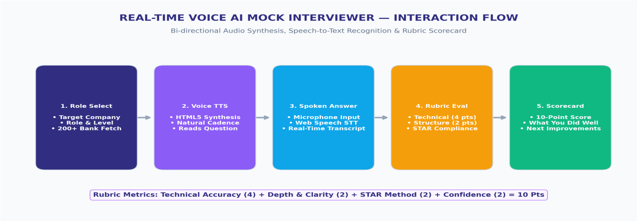
Figure 4: Bi-Directional Speech Synthesis (TTS) & Speech Recognition (STT) Interview Pipeline
